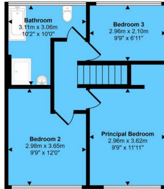
First Floor Approx 42 sq m / 453 sq ft
