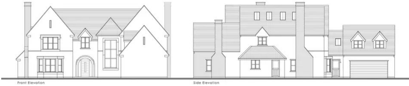
Front Elevation
